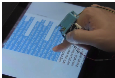
Figure 5. Select+Scroll- Index finger used for selecting and the thumb controls the scrolling.
