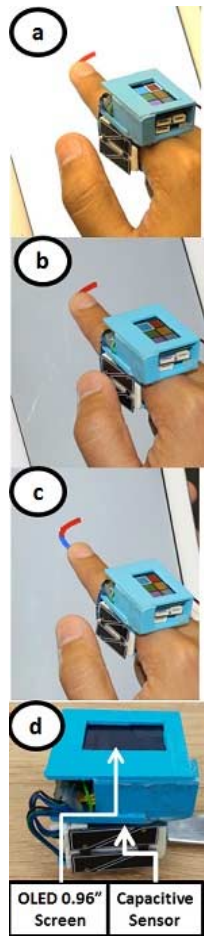
Figure 1. Workflow of Ringteraction. (a) The user is drawing in red; (b) by tapping on the capacitive sensor of the ring with their thumb, they change the color to blue and (c) start drawing in blue. (d) Hardware details of our prototype.
